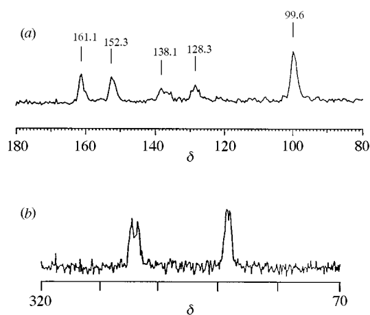
Fig. 1 (a) 50.32 MHz ^{13}\text{C} CP MAS NMR spectrum of 2 recorded at room temperature (300 K): 7 s ^1\text{H} -90° pulse width, 4 ms contact pulse, 5 s repetition time, spectral width 20 kHz; (b) room temperature (300 K) 9.12 MHz ^{15}\text{N} CP MAS NMR spectrum of 2 : 5.5 s ^1\text{H} -90°, 5 ms CP-time, 4 s recycle delay, spectral width of 7 kHz, no line broadening used
